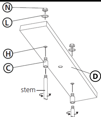
Drawing 2 – Canopy Assembly
